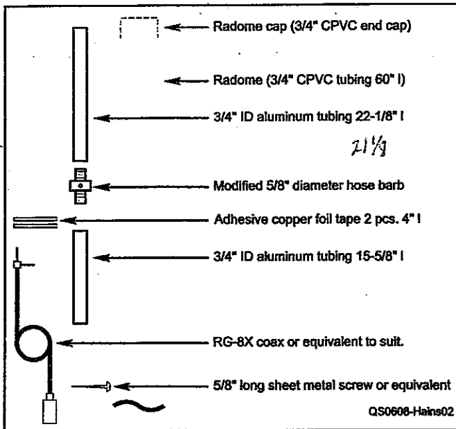
Figure 2 — The components of N1GY's version of the antenna.
