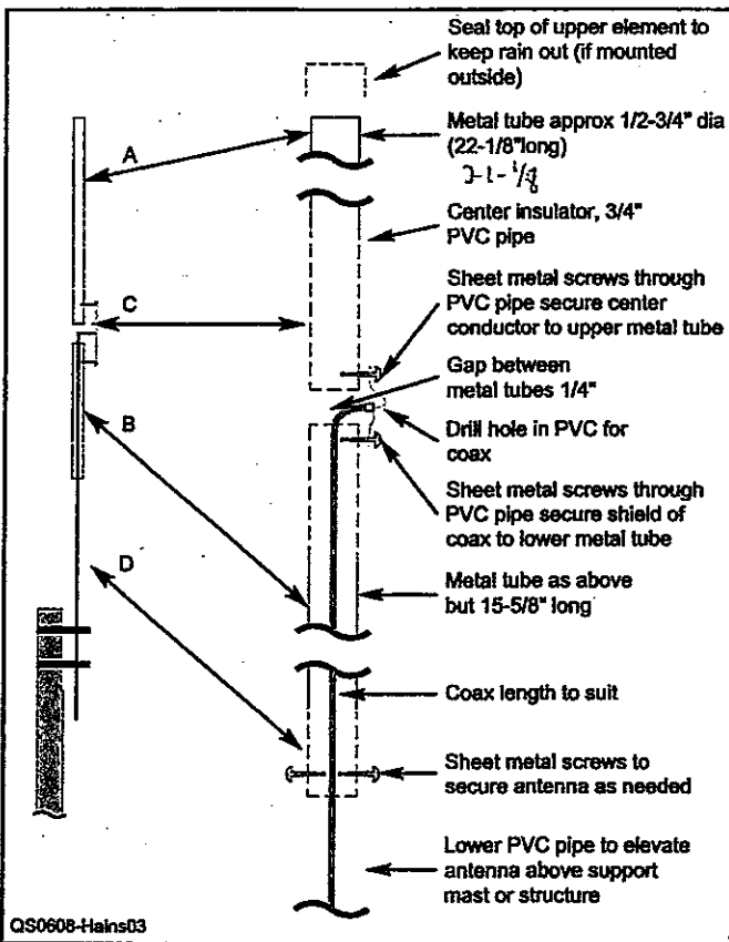
Figure 3 — Details of radome construction.
