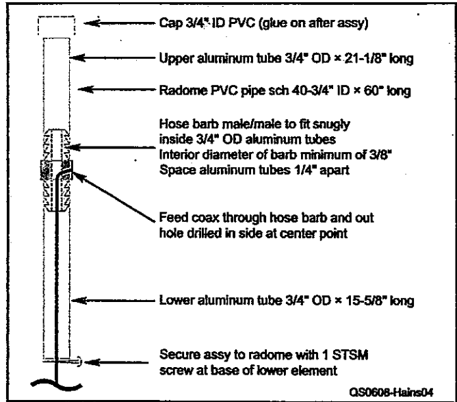
Figure 4 — Details of antenna installation in radome.
